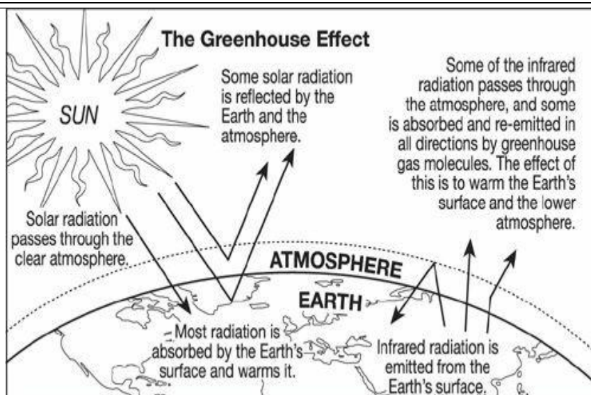
10. The greenhouse effect
